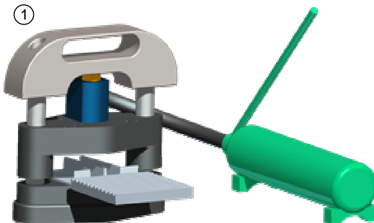
① Punching of the open finger joint with hydraulic punching machine
