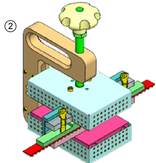
② Welding of the tapered fingers with mobile welding press
